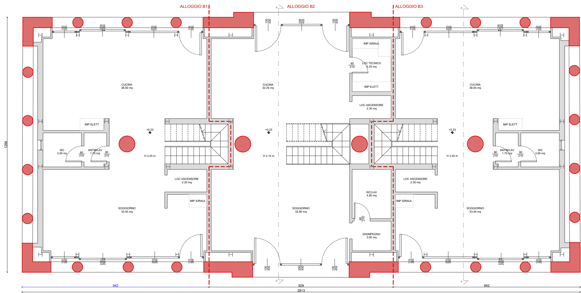
PLANIMETRIA PIANO TERRA
